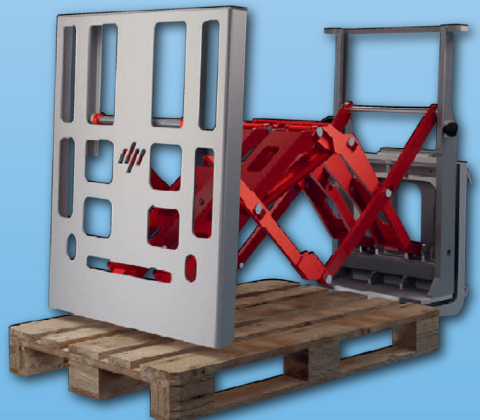
Pusher AS, available in different versions
