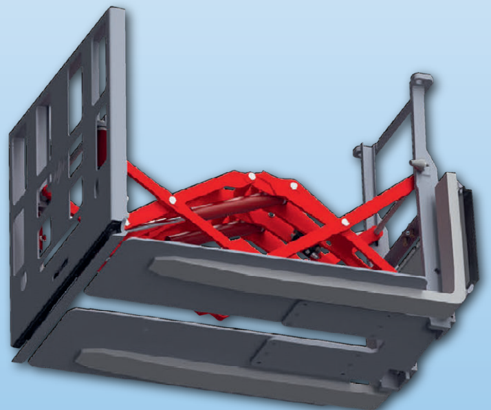
Bottom view KA installed on forks
