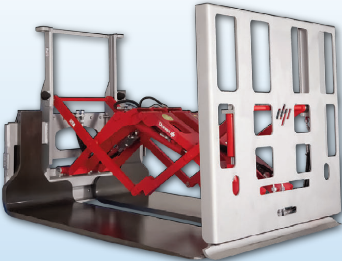
Carriage mounted push pull KA-ISO
