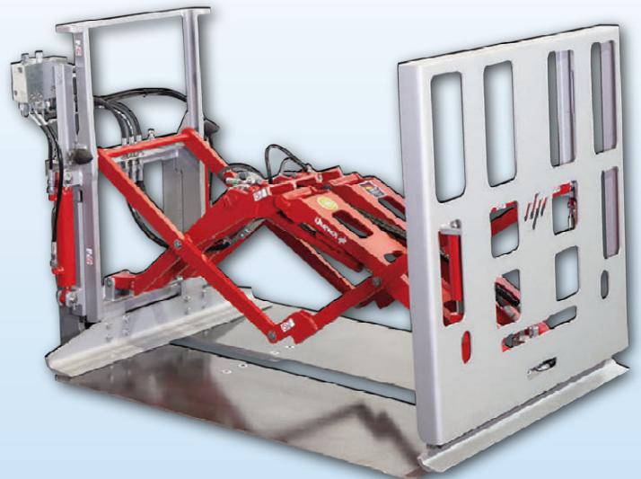
Fork mounted push pull KA-GZ-P with sheet saver
