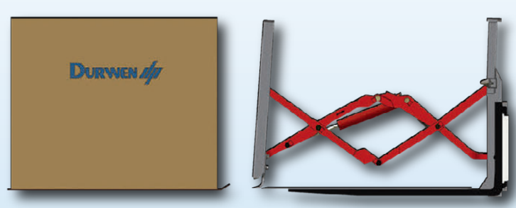
Goods on slip sheet
