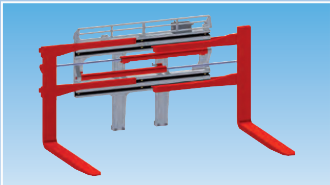
ZVP-H for reach trucks, without sideshift, with bolt-on forks, wide frame, extra ground clearance for wheel legs
