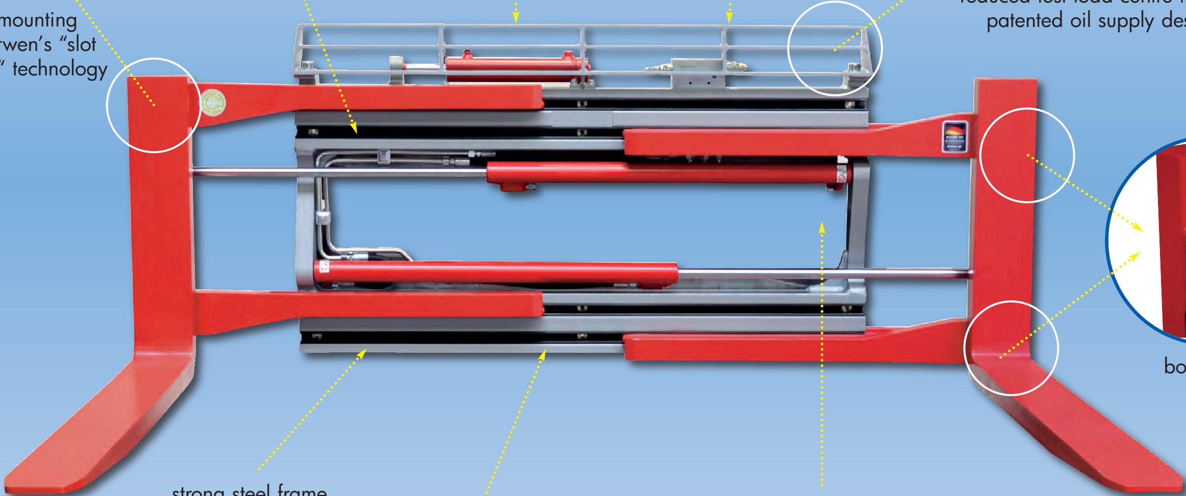
compact design gives excellent visibility
