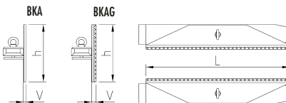
slip-on arms for bales
