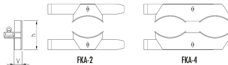
slip-on arms for drums (for safe transport of drums)
