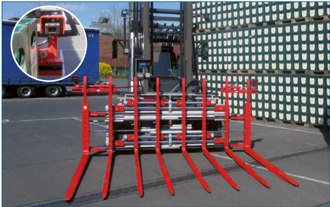
image shows APK 80-C with special equipment: telescopic camera
