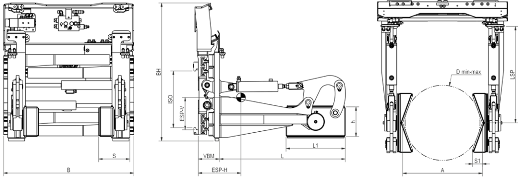
Tilting drum clamp 90°, with integral sideshift
