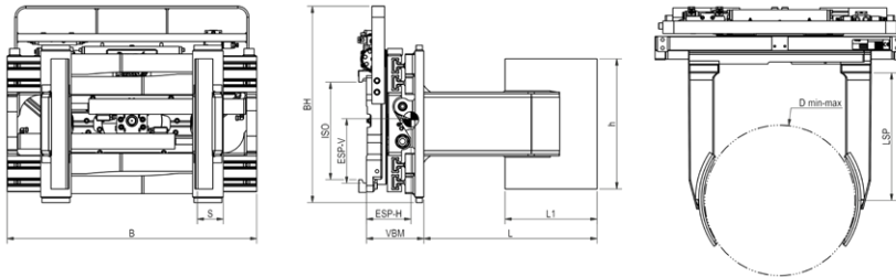
Revolving drum clamp without sideshift
