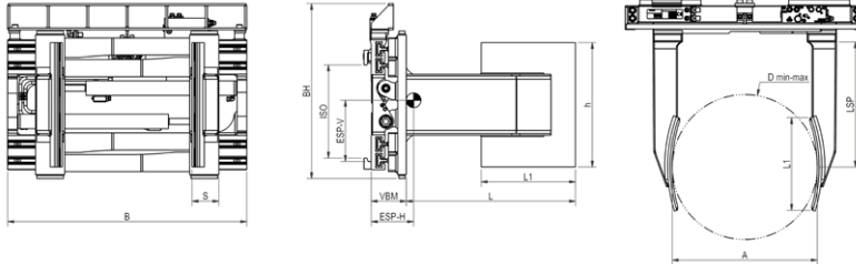
Drum clamp with integral sideshift
